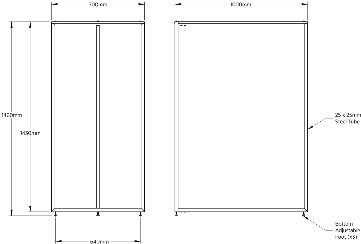
■ Assembly 65 – 700 x 1000
